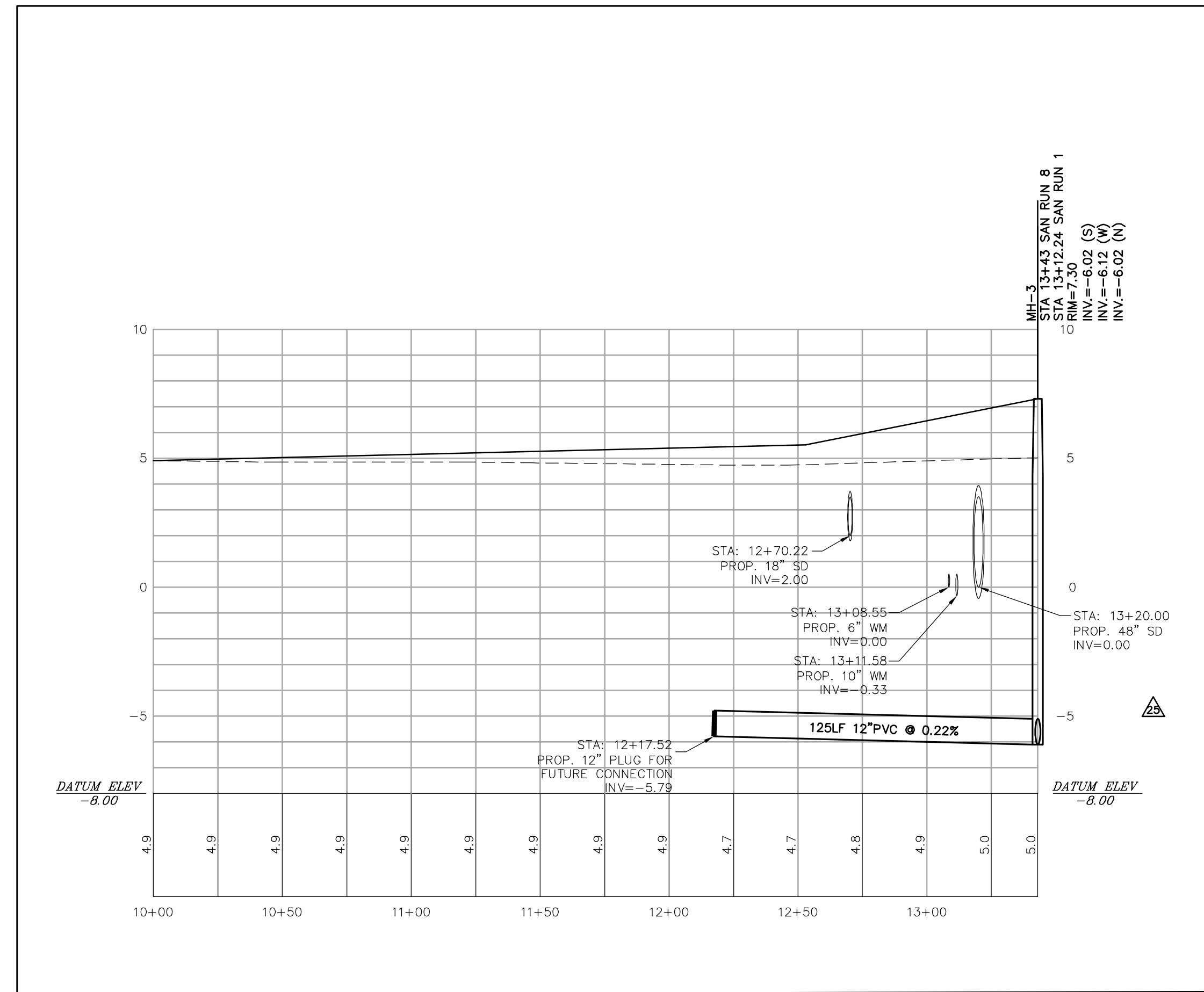
SANITARY PROFILE 8 HORIZ. SCALE = 1:40 VERT. SCALE = 1:4
