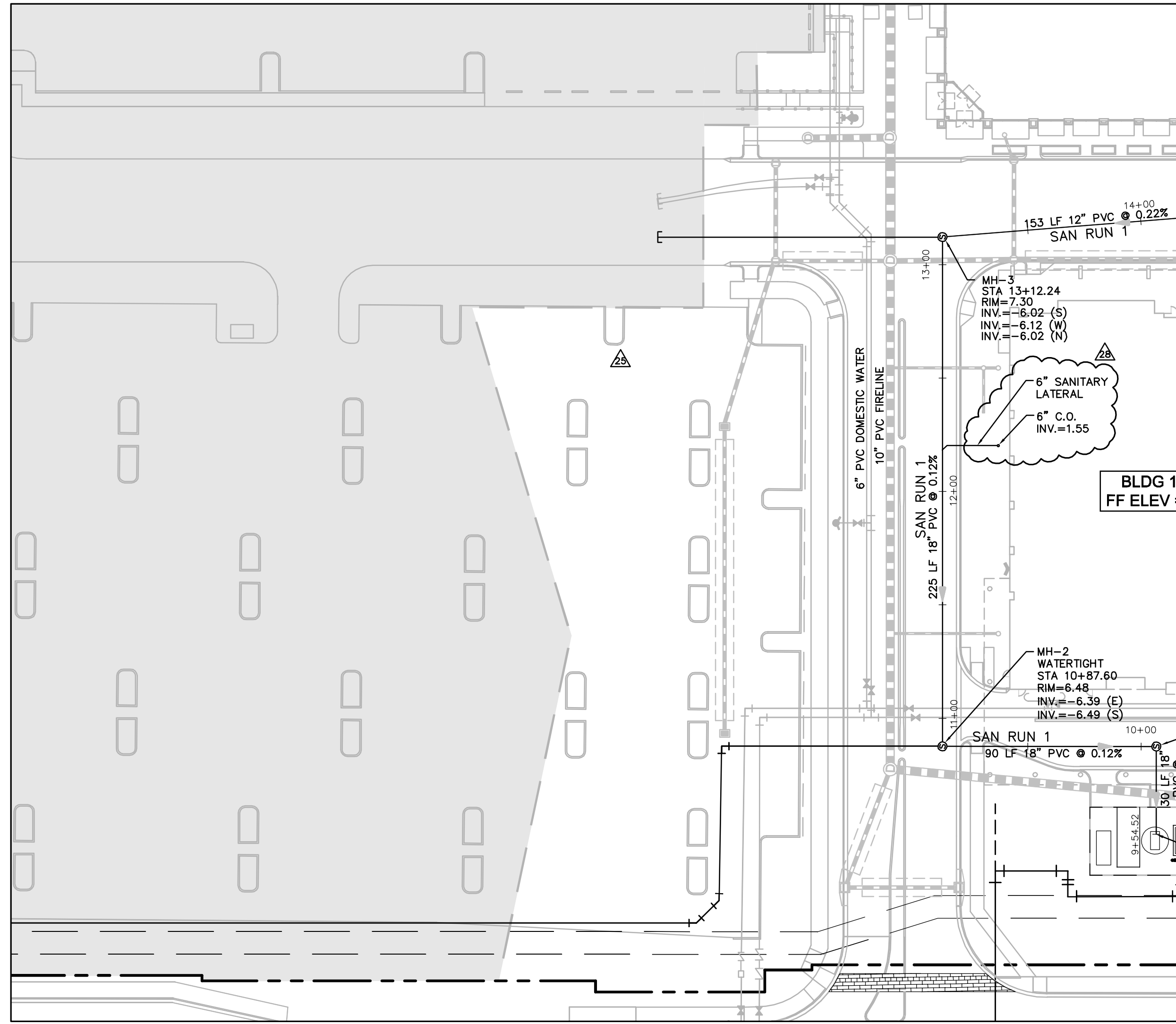
SANITARY PLAN 8
